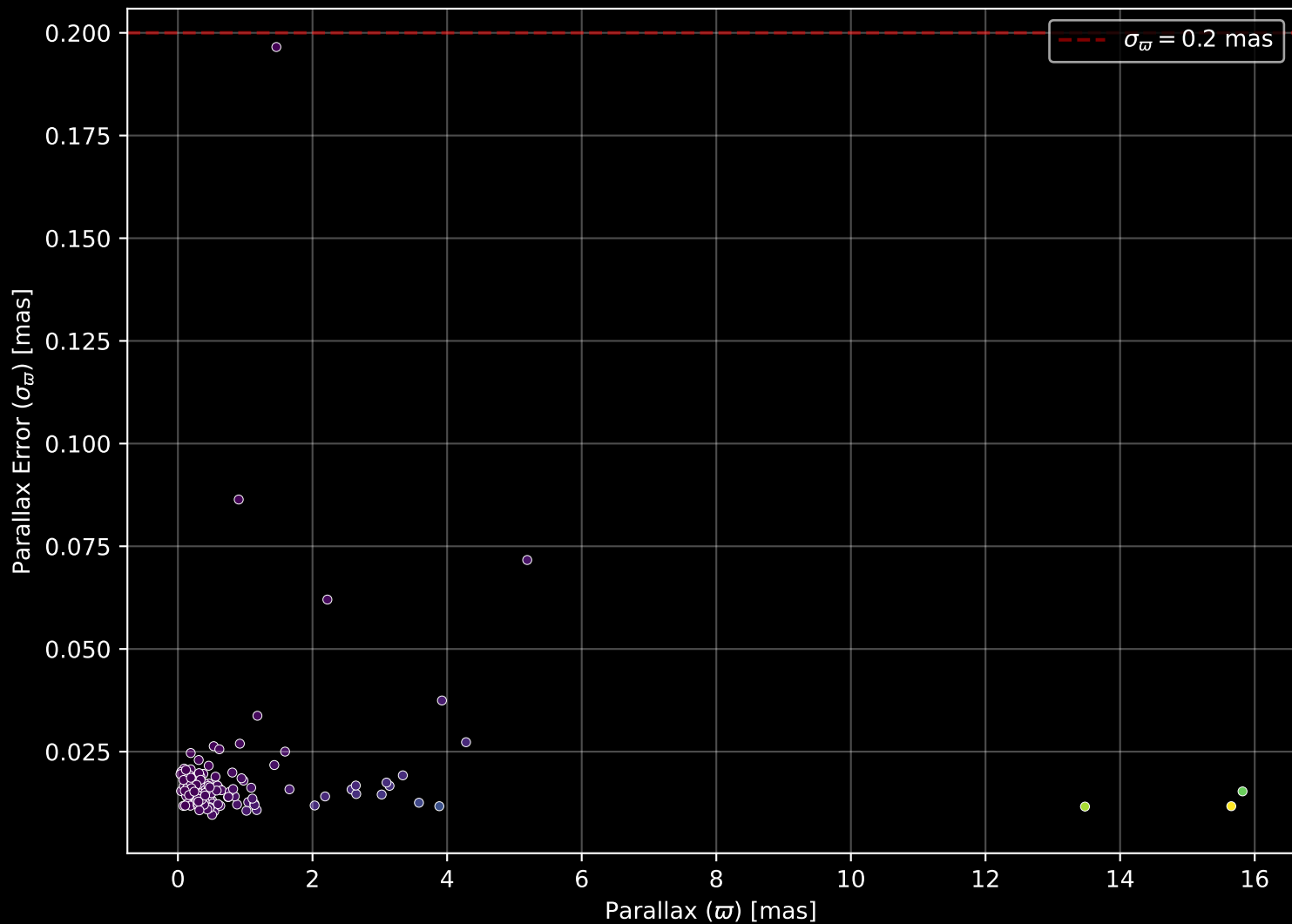
APOGEE DR17 Field: [105-12] Parallax Quality (n= 140)
