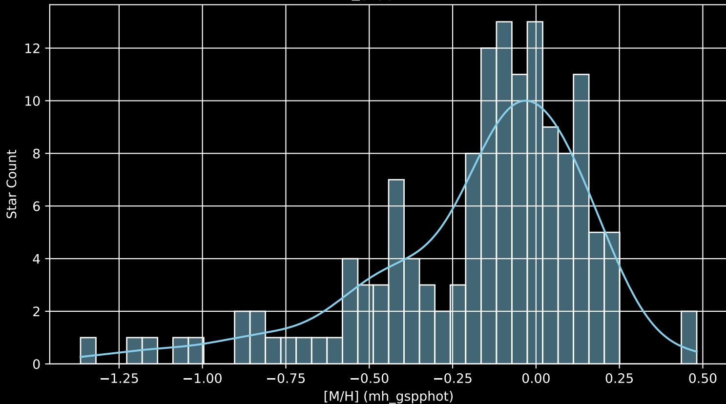
APOGEE DR17 Field: [105-12 [M/H] (mh_gspphot) (n= 140)
