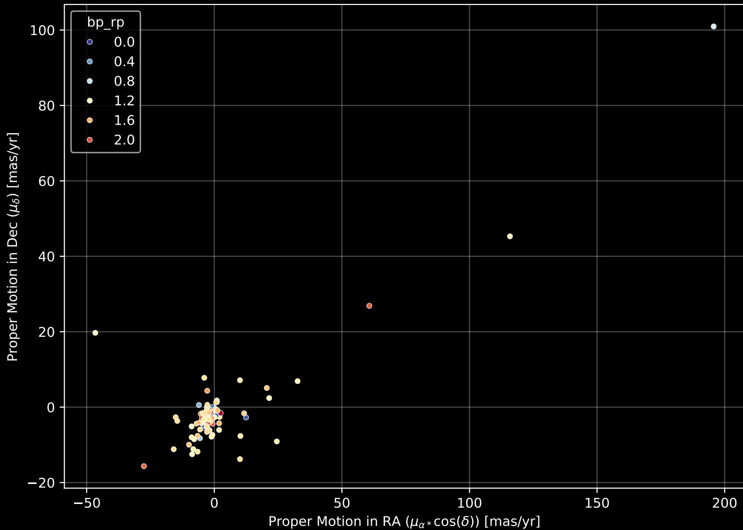
APOGEE DR17 Field: [105-12] Proper Motion Diagram (n= 140)
