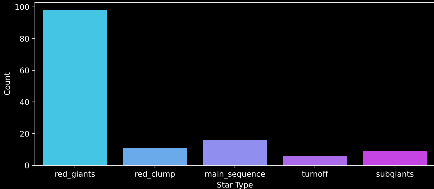
APOGEE DR17 Field: [105-12] Count plot of Star Type
