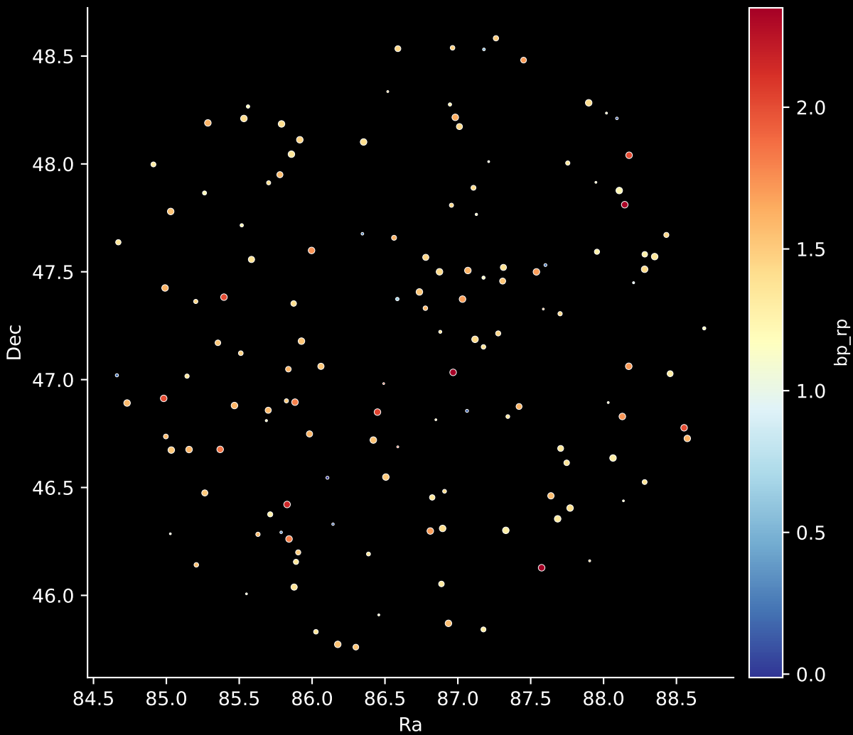
APOGEE DR17 Field: [105-12] Stars: 140
