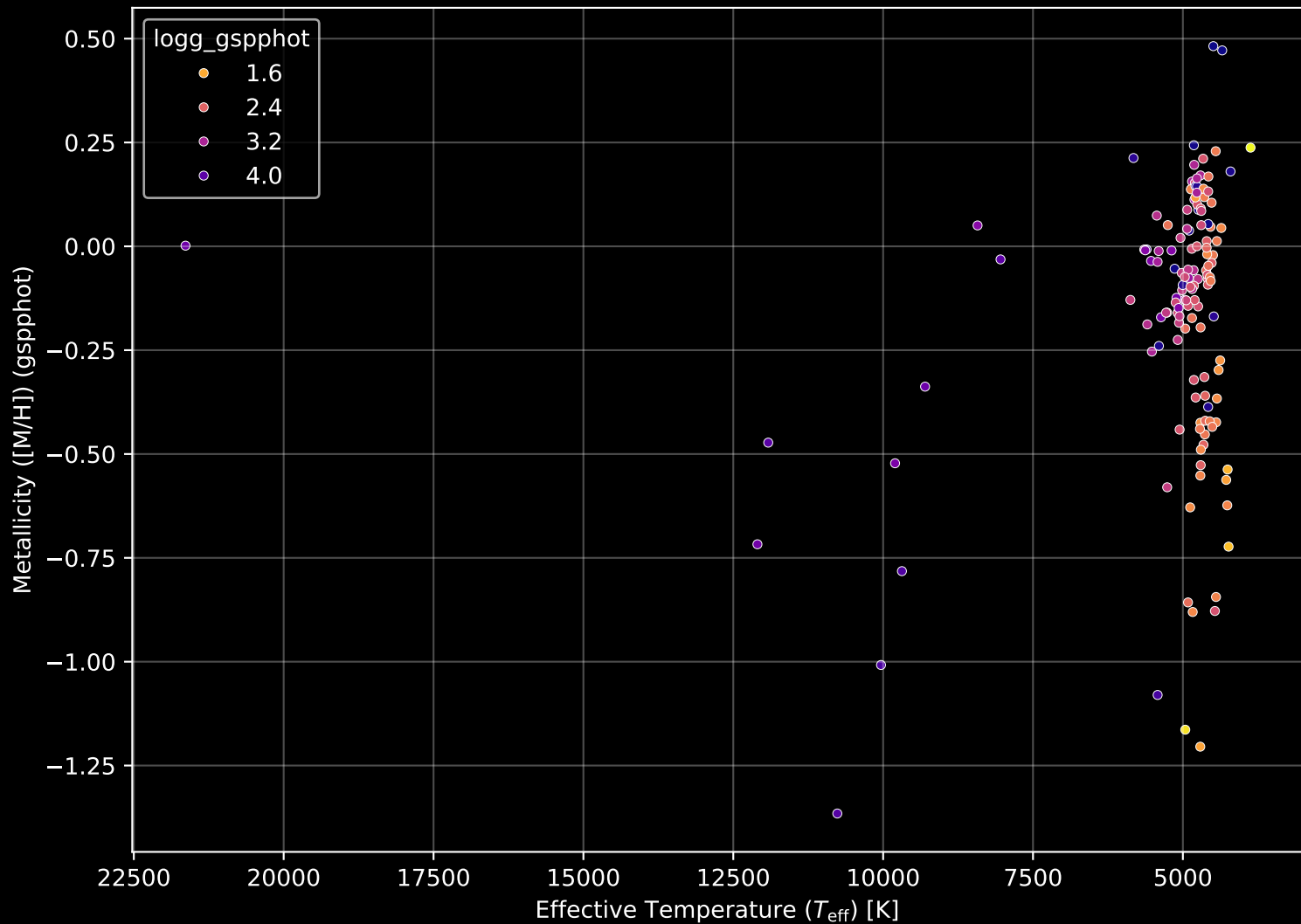
APOGEE DR17 Field: [105-12] Stellar Population Parameters (n= 140)
