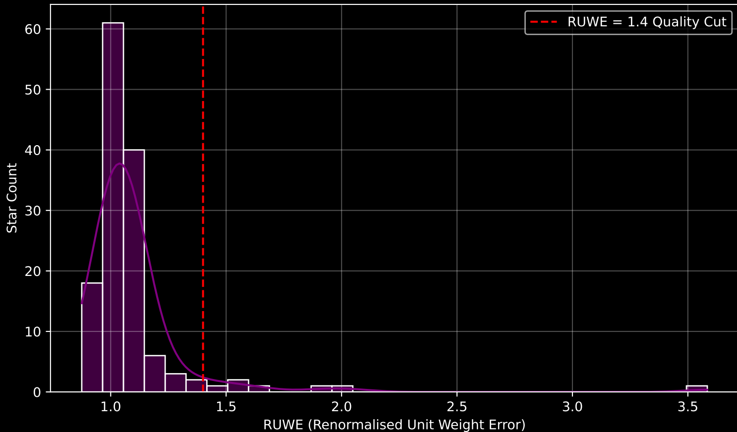
GAPOGEE DR17 Field [105-12] RUWE Distribution (n= 137)
